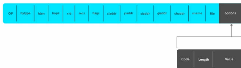
Figure 31. DHCP packet Format
